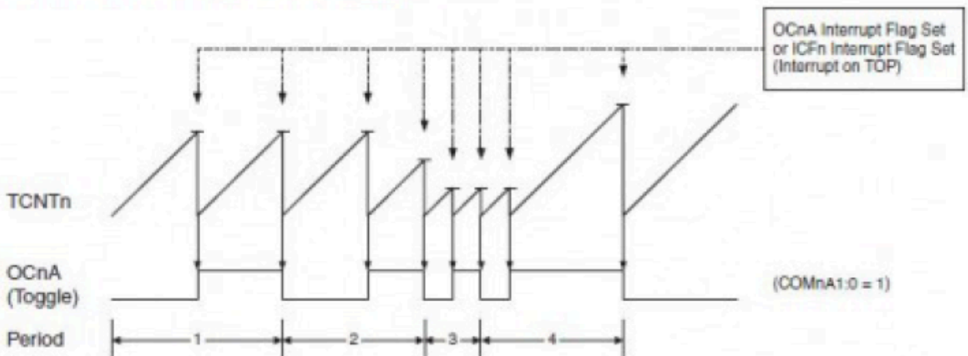
Figure 16-6. CTC Mode, Timing Diagram
